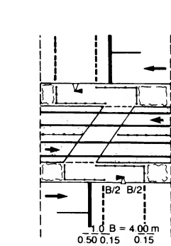
7 Permanent pedestrian crossing without signals
